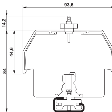
Dimensional drawing
